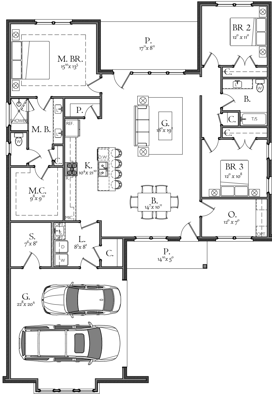
MAIN LEVEL
