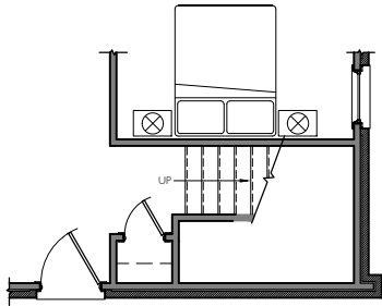
STAIR LAYOUT FOR BONUS
